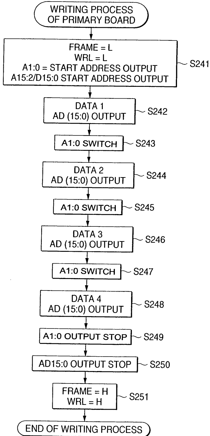
FIG. 23 PRIOR ART
